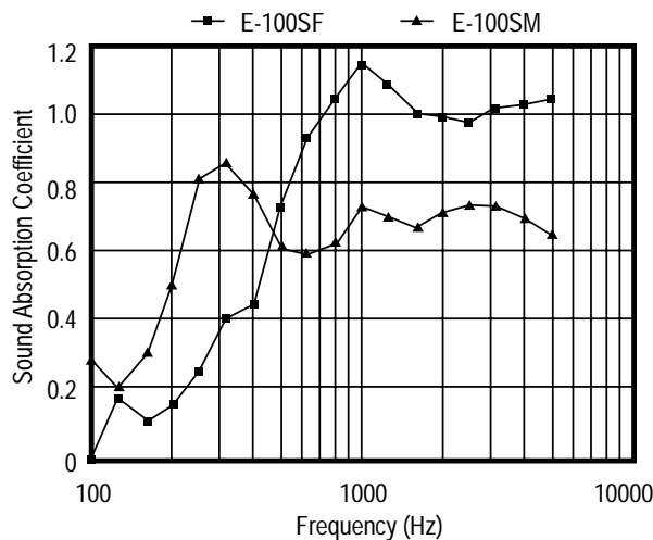
Figure 3: Performance of Various 1-inch Acoustical Foams with Surface Treatments
