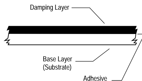
Figure 6: Extensional (Free-layer) Damping Construction, Cross Section
