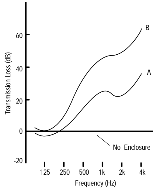
Figure 4: Insertion Loss of Sealed Enclosure without Absorption (A) and with Added Absorption (B)
