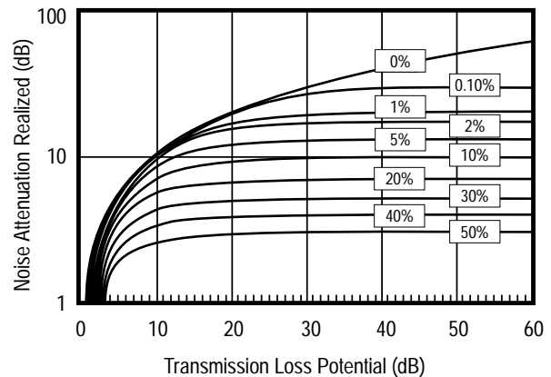
Figure 2: Performance of an Enclosure Based upon Percentage of Open Surface Area
